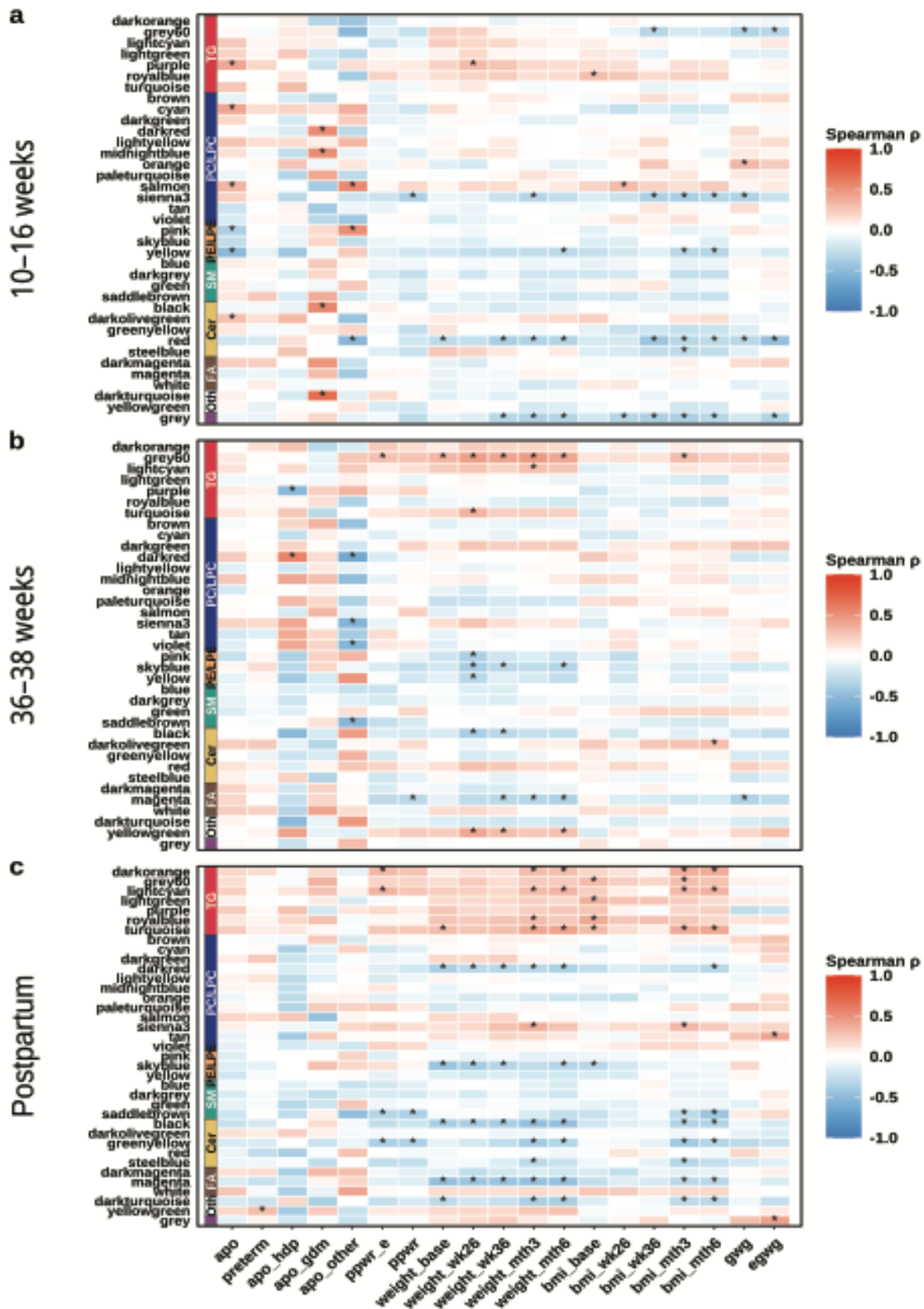
Figure S – Module-Trait Correlation with covariates adjusted (age, BMI at signup, race, group)
