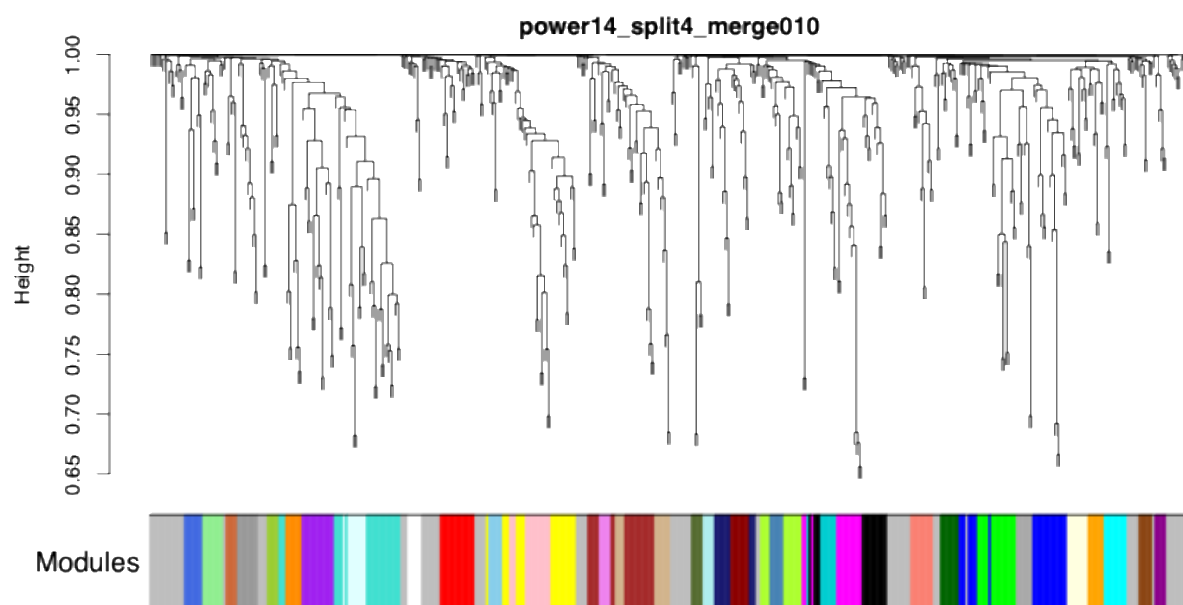
Figure S2 - Cluster Dendrogram of module distribution
