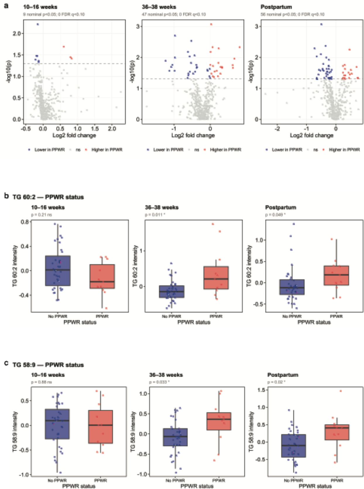
Figure S – Differential lipid analysis APO 48 samples
