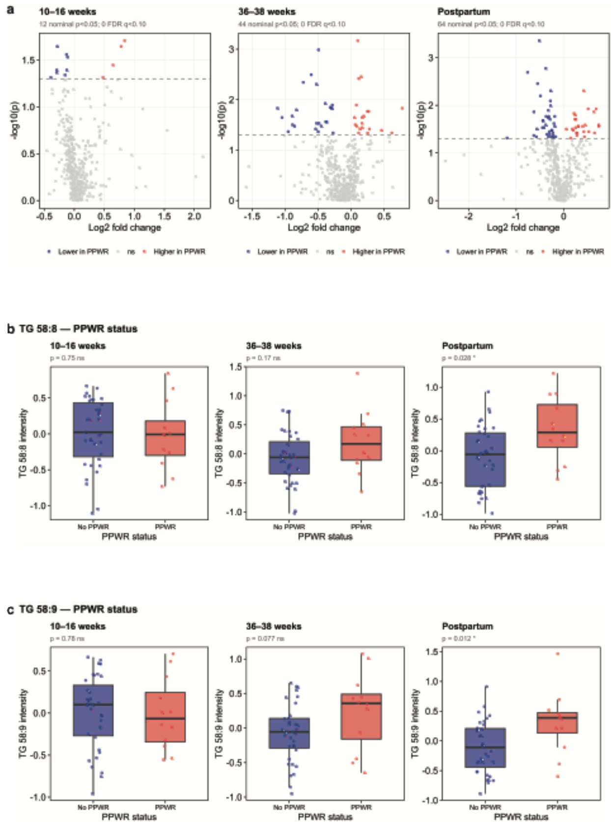
Figure S – Differential lipid analysis PPWR full
