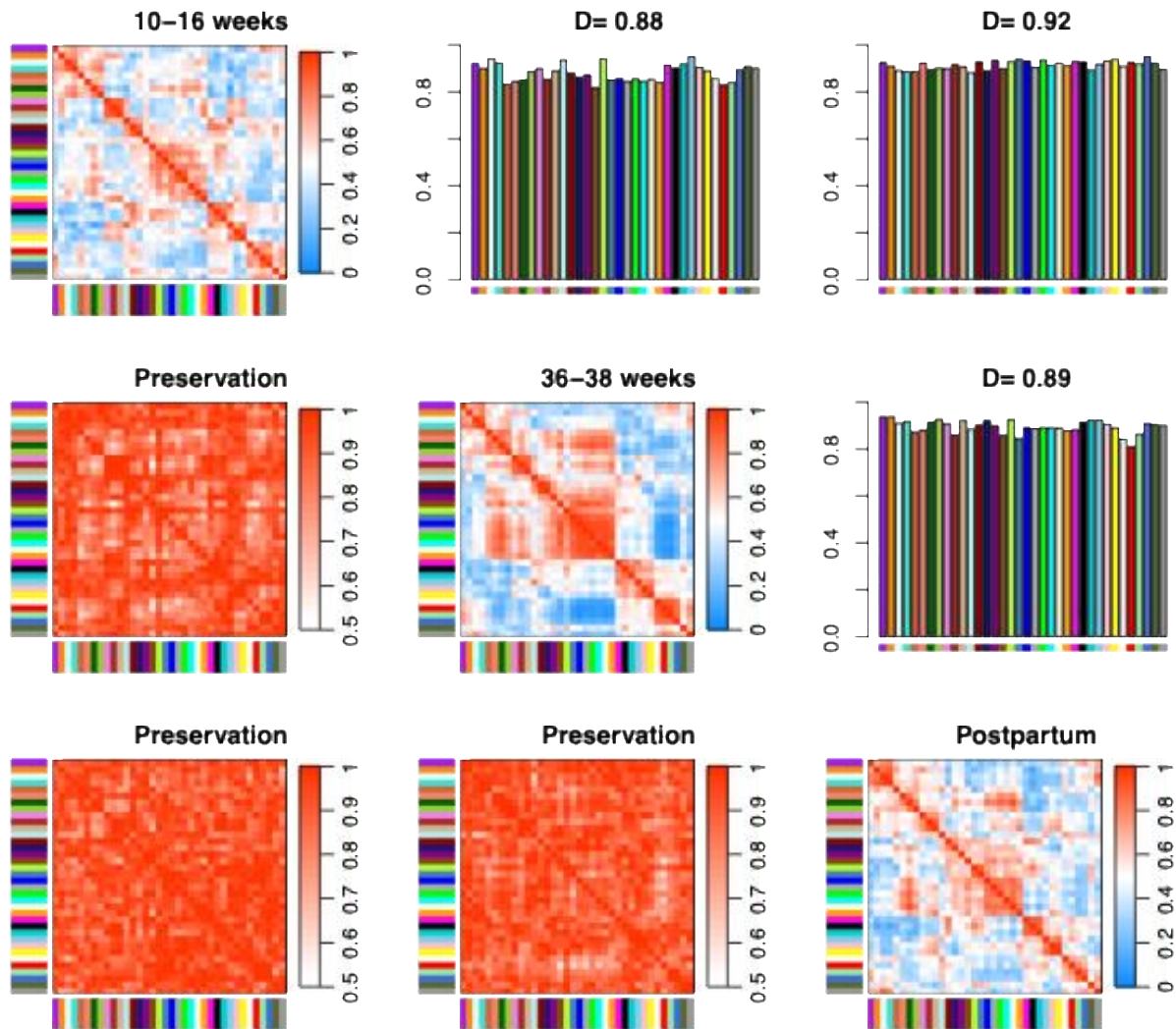
Figure S6 – Consensus modules similarity and module preservation
