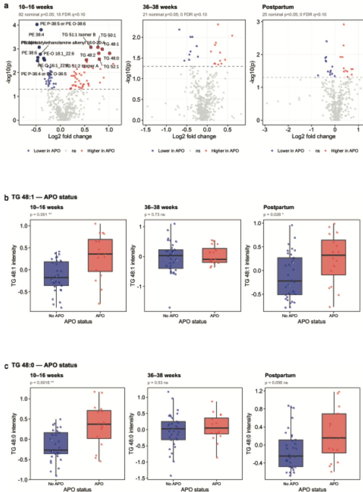
Figure S – Differential lipid analysis APO full
