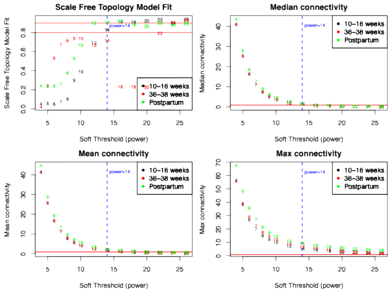
Figure S1 - Soft power threshold calculation
