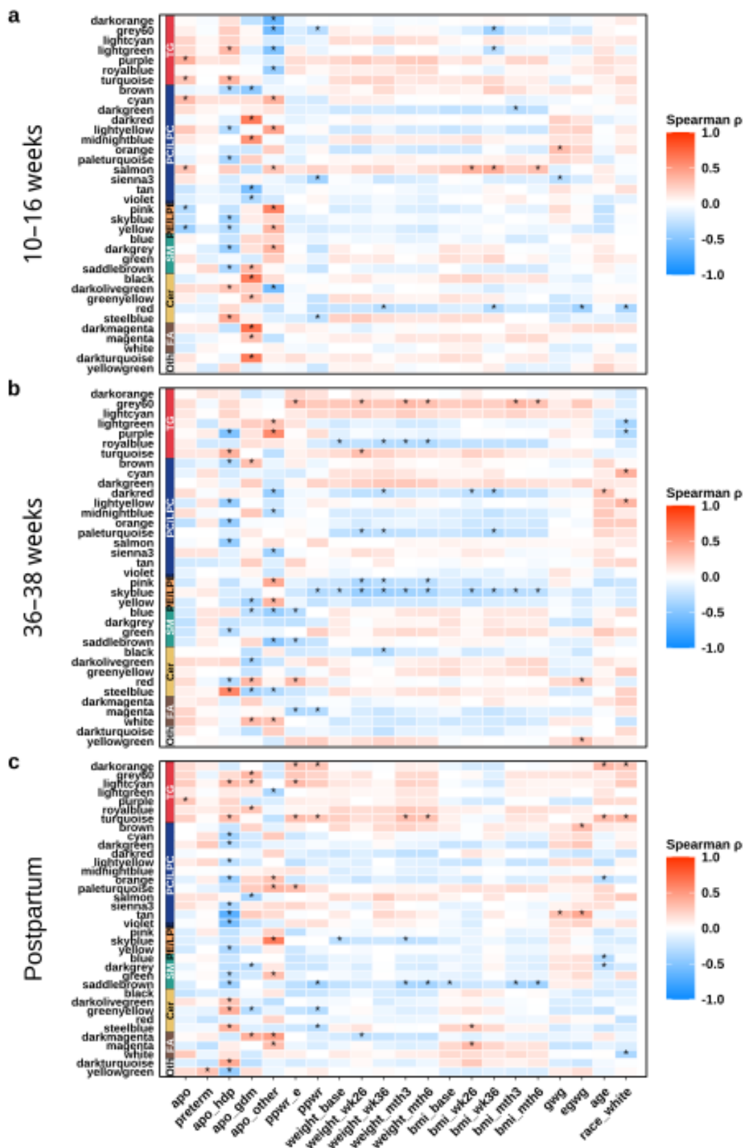
Figure S – Module-Trait Correlation with intervention group adjusted
